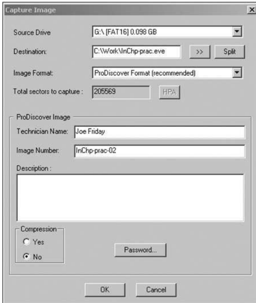
Figure: The completed Capture Image dialog box
