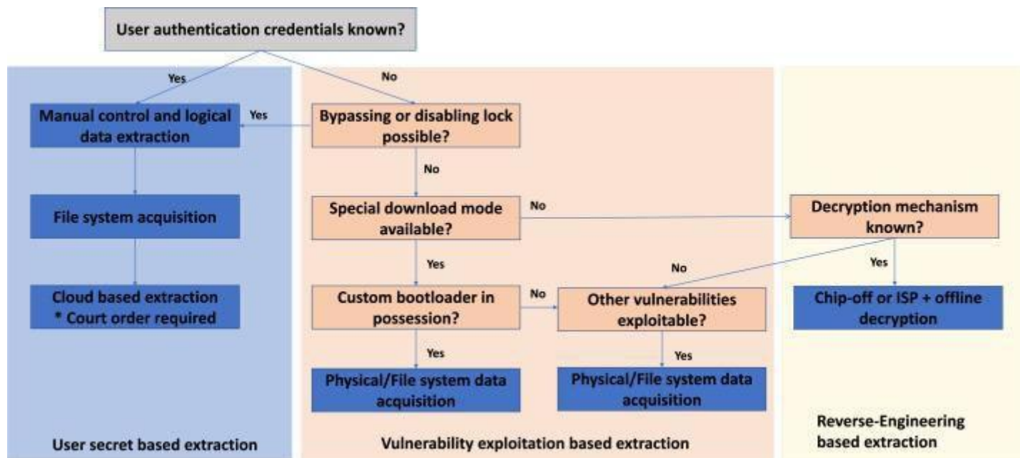
Figure: New mobile forensic data extraction model.
